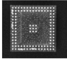
BGA Inverted
