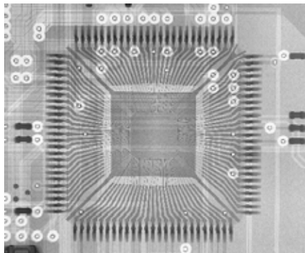
QFP
