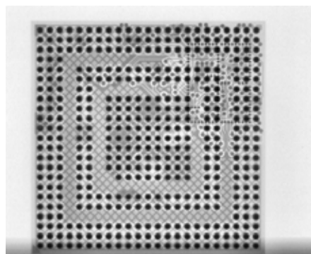
BGA
